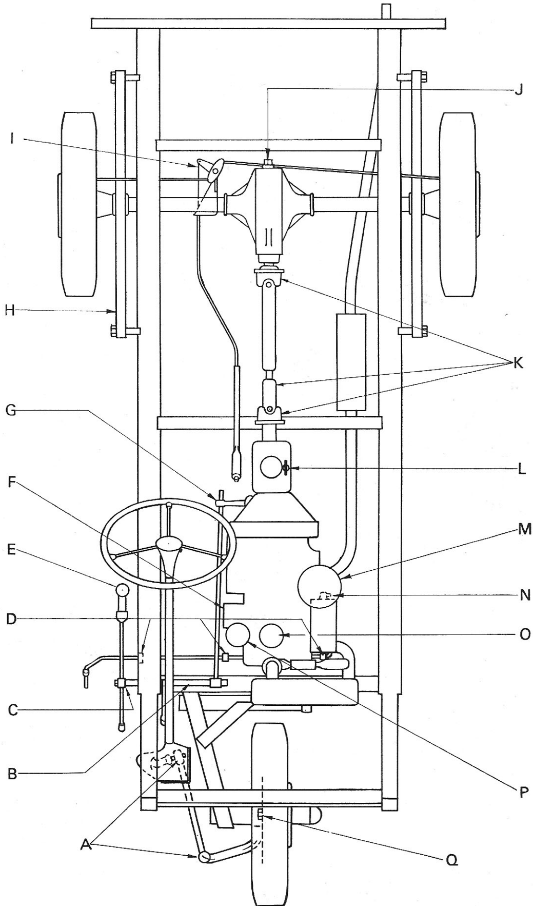
Figure 42 Lubrication points
